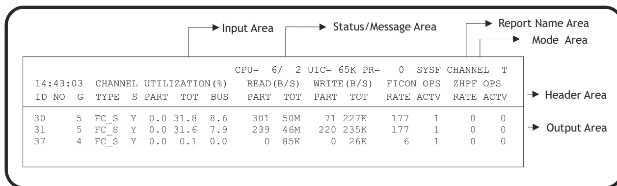
Figure 34. CHANNEL report as example of a Monitor II report header (TSO/E session)
